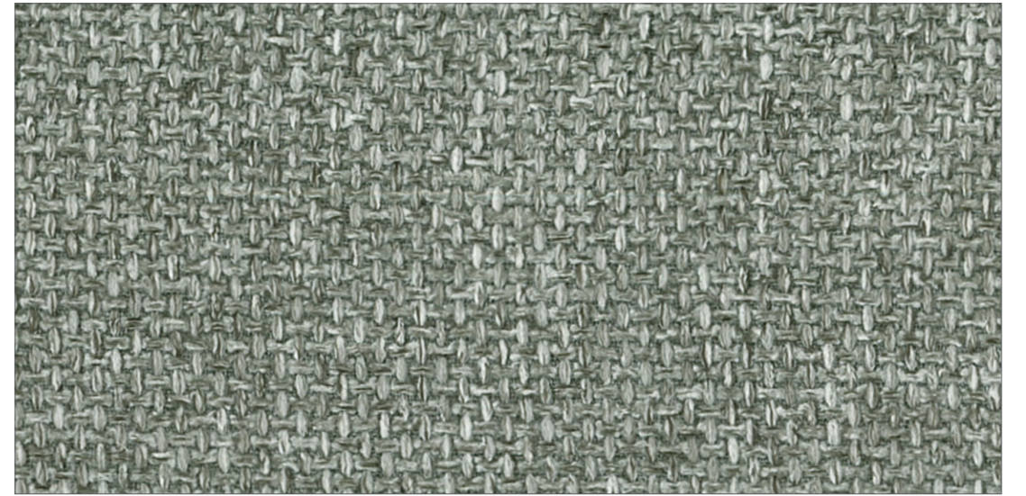
Glacier
