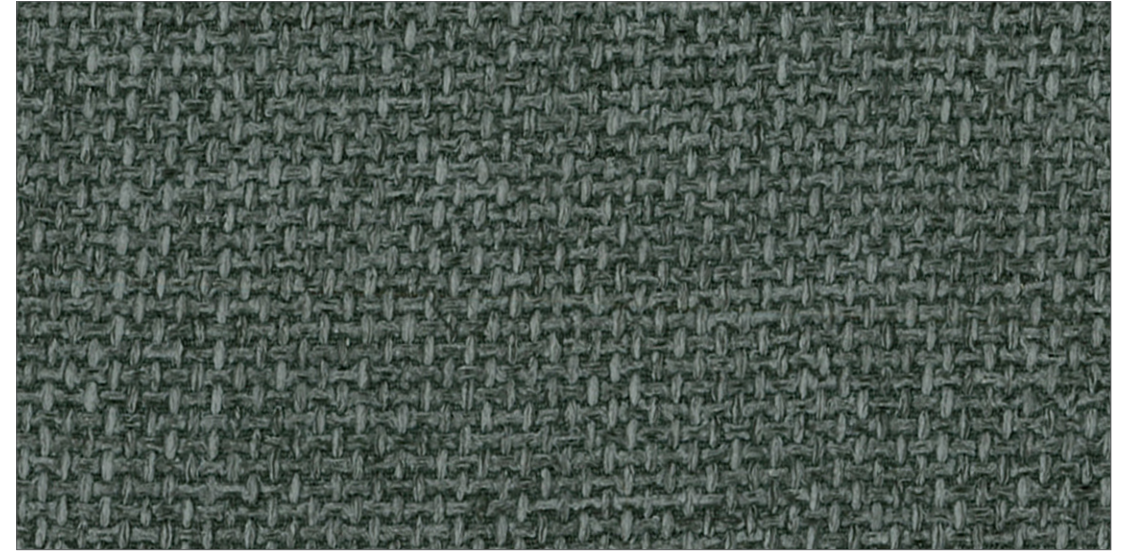
Coal
