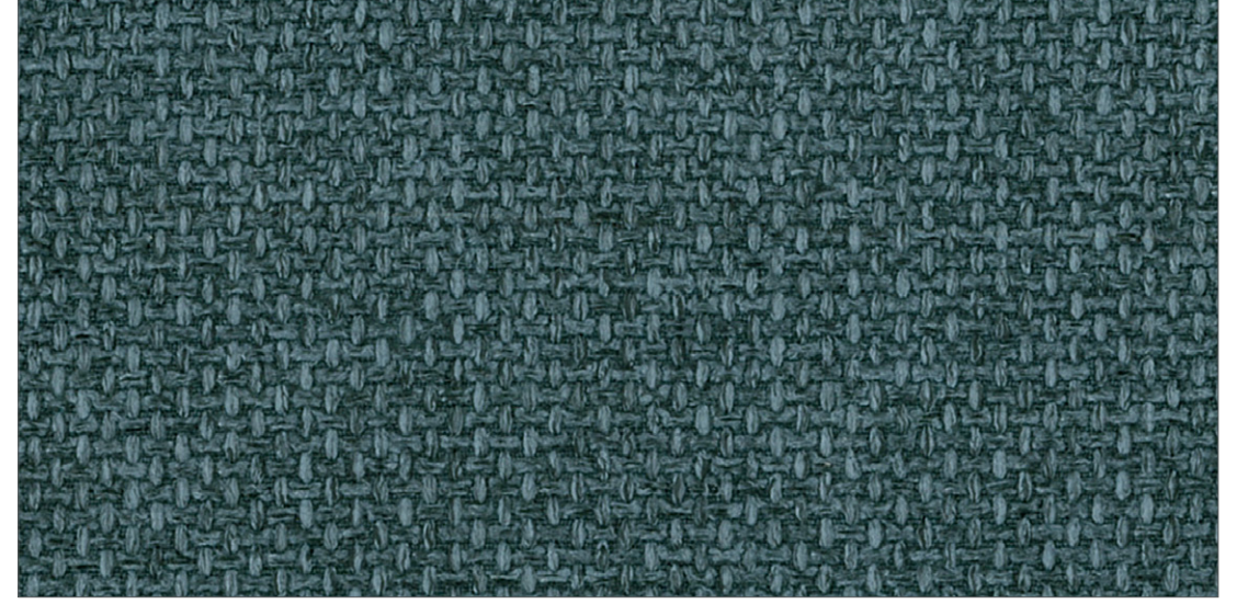
Ocean
